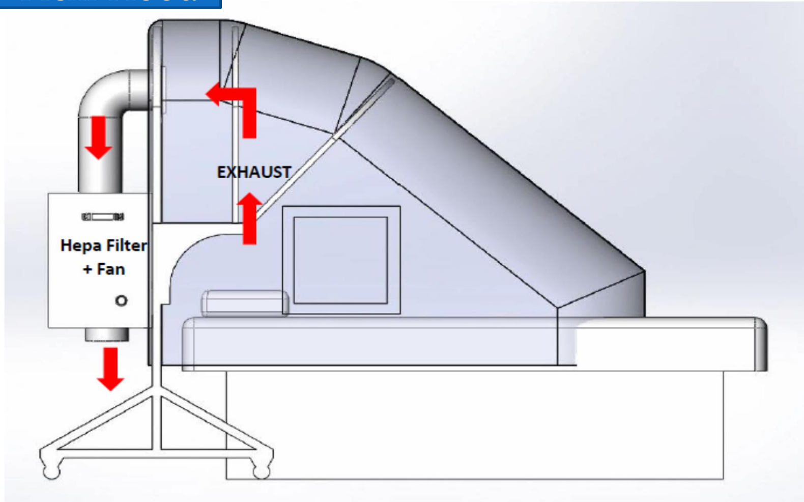
Flexi Hood
